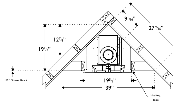
MQ19ZDV Corner Framing Dimensions (inches)
